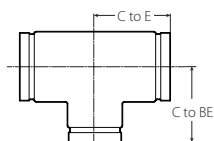
Molded
