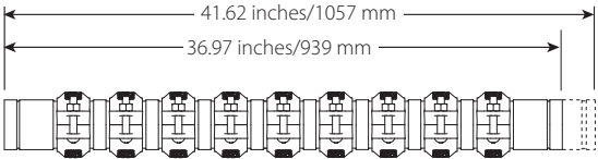
4-inch/DN100 Style 355/355P Expansion Joint
