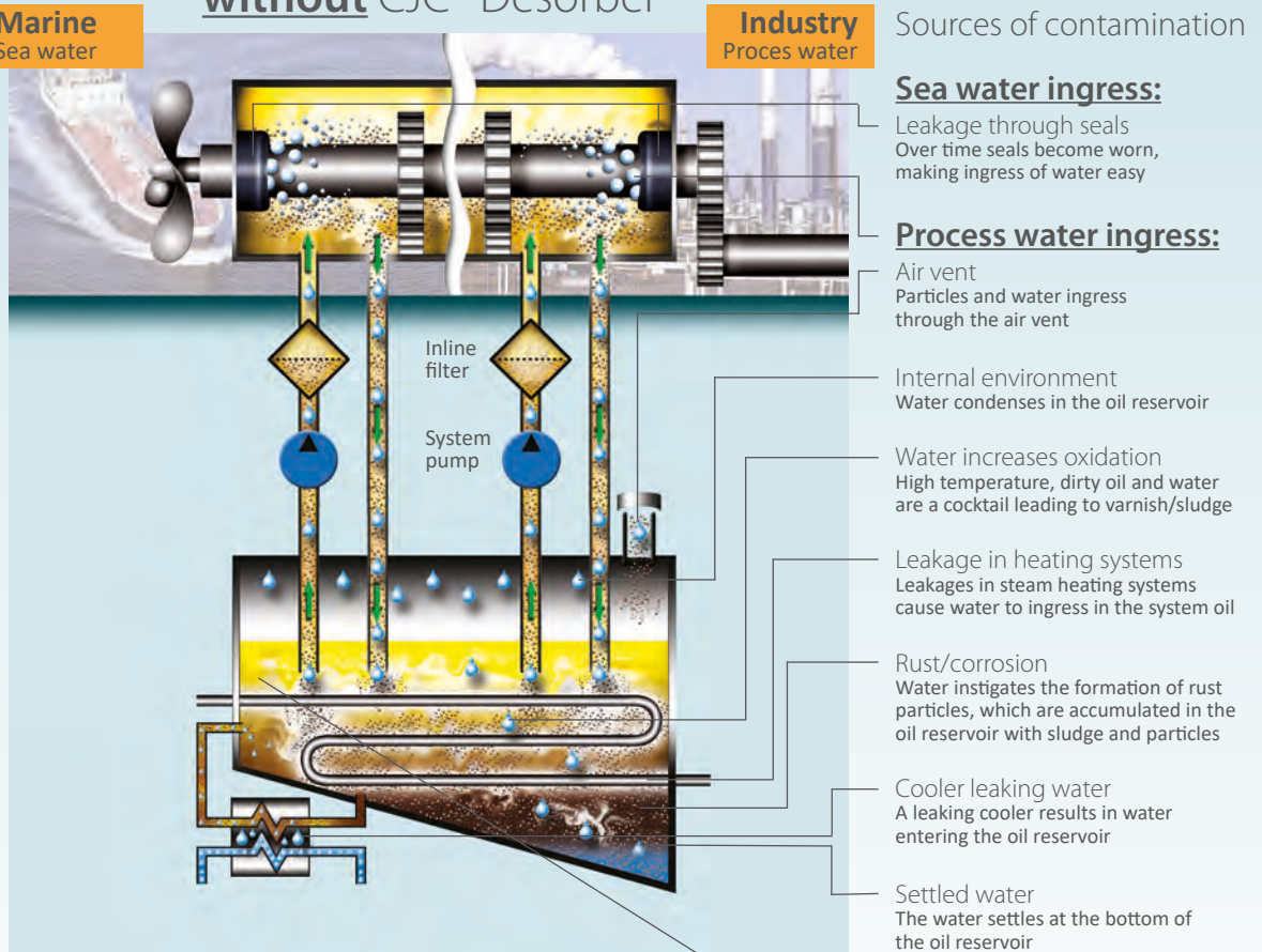
Water contamination on steel mill/ gear
